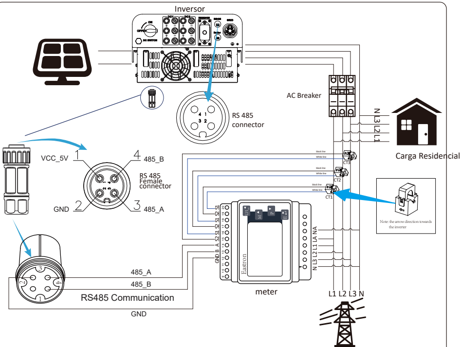
Eastron SDM630MCT Figura 7.12 Medidor Eastron
