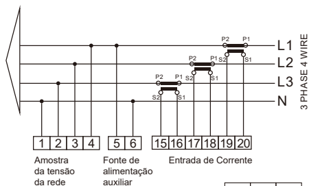
Eastron SDM630MCT Figura 7.12 Medidor Eastron
